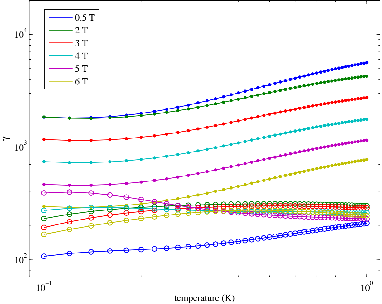
Figure 3.1: Theoretical calculations of the Al- ^3\text{He} collision rate ratios for ^2P_{1/2} state m_J -changing (●) and ^2P_{3/2} state J -changing collisions (○) by Tscherbul [95]. Both values of \gamma reflect the ratios of the ground-state momentum transfer rate coefficient to the respective inelastic collision rate coefficients. The dashed line is the experimental temperature.
