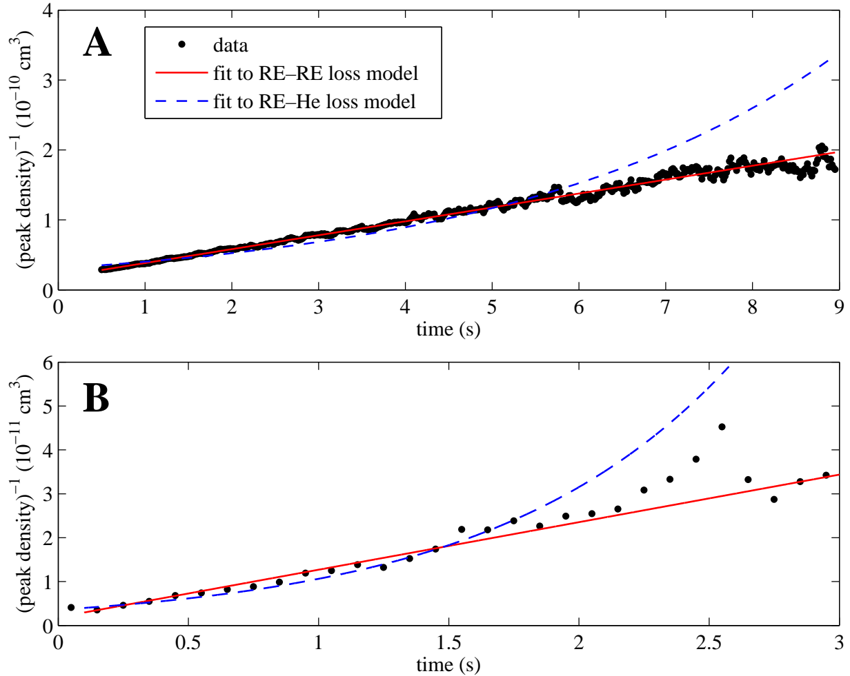
Figure 4.6: Decay of trapped (A) erbium and (B) thulium. The vertical axis is the reciprocal of the peak atom density determined from spectra. The solid red line is a fit to Equation 4.6, for decay only from RE-RE collisions. The dashed blue line is a fit to the exponential decay expected for loss only due to collisions with a constant helium density. The excellent fits to Equation 4.6 indicate that the atom loss is due to RE-RE collisions.
