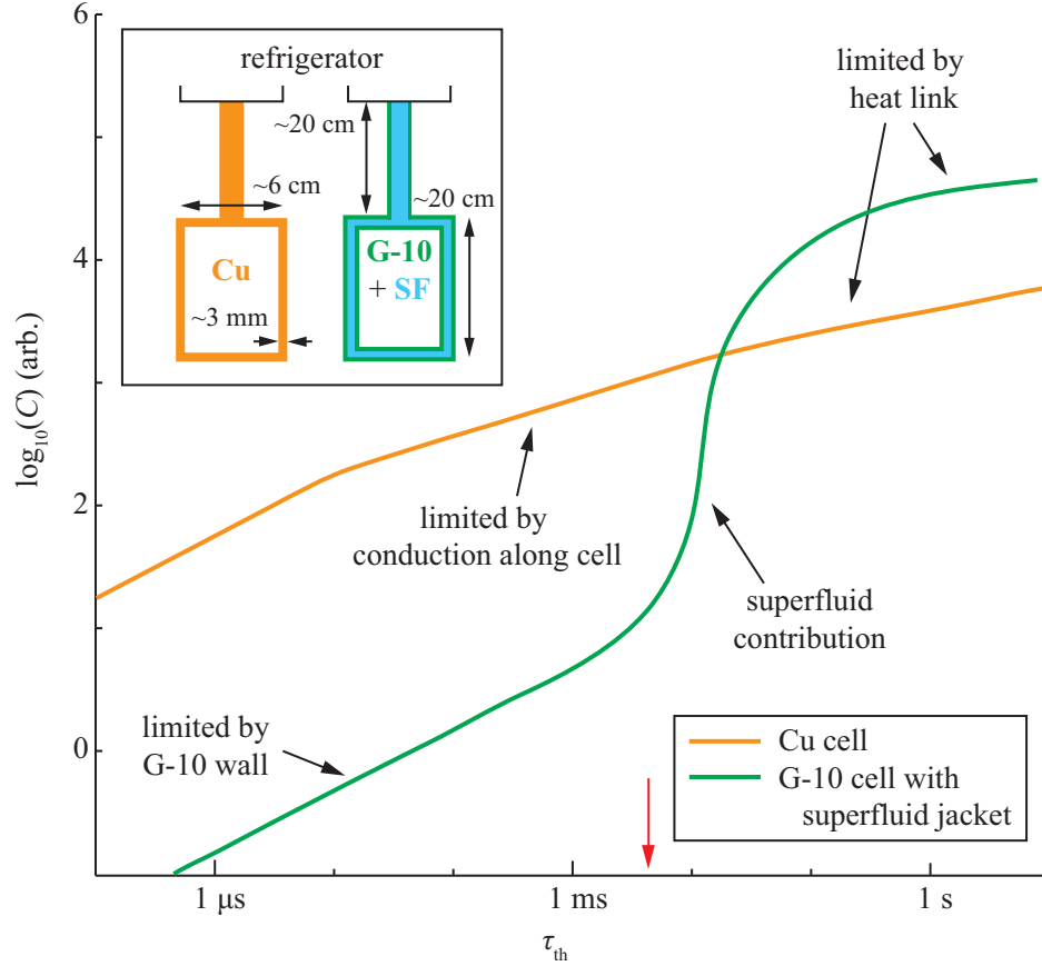
Figure 2.5: Sketch of thermal behavior of copper vs. superfluid-jacketed G-10 cells for a simplified model cell with some dimensions shown. The heat capacity C available to absorb energy (such as that used for ablation production of Sb) is given as a function of the time necessary for diffusing heat to reach that heat capacity. A larger value of C implies a cooler temperature. Over short timescales, heat can reach only the inner wall of the cell, but over long times the entire cell, heat link and refrigerator contribute. The low thermal conductivity of G-10 implies a low C for timescales \lesssim 10\ \text{ms} . However, the very large conductivity and specific heat of superfluid helium dramatically changes the behavior beyond this time. The red arrow indicates the average ballistic cell transit time of Sb at 800 mK. This diagram is approximate and highly dependent on temperature and geometry. The effects of the cell window and other “hot spots” have been ignored.
