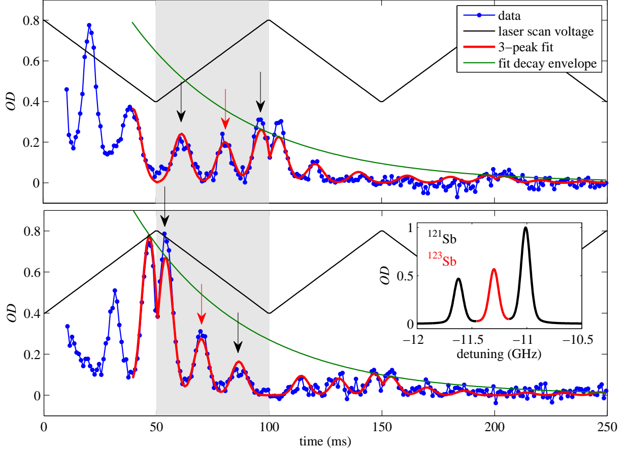
Figure 2.14: Measurement of the Sb 4S_{3/2} \rightarrow 4P_{5/2} isotope shift. The laser is scanned over 3 peaks (a single scan is highlighted in gray), which simulation of the hyperfine spectrum identifies as the m_F = 2 \rightarrow 3 and 3 \rightarrow 3 transitions of ^{121}\text{Sb} (black arrows) and the m_F = 2 \rightarrow 1 transition of ^{123}\text{Sb} (red arrow). The laser can only be stably scanned over this range at \leq 10 Hz, so there is significant spectral distortion due to diffusive decay ( \tau_d \approx 50 -ms). The scanned data trace is fit to a 3-peak spectrum (inset) repeated at the scan rate within a decaying exponential envelope (dashed green). To mitigate nonlinearity in the laser scan, the measurement is repeated with the scan phase shifted by 180^\circ . The two results bound the measurement confidence interval and are averaged to give a final value of \Delta\nu_{123-121} = 273(10) MHz.
