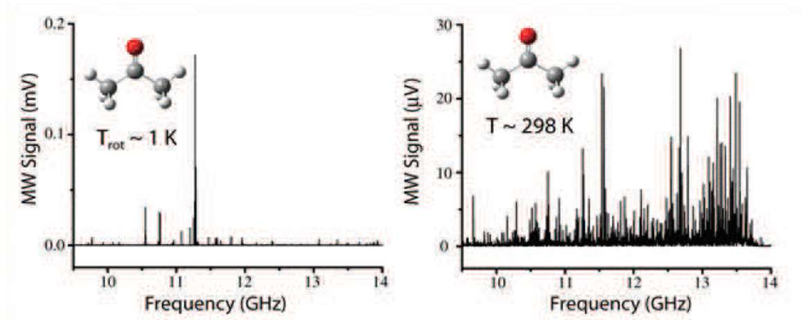
Spectra from Pate group, UVA
