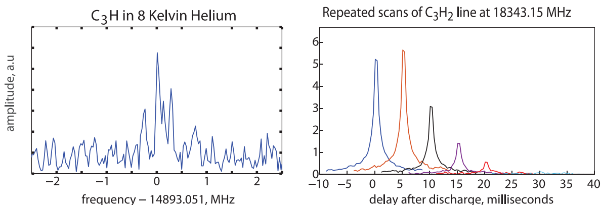
Figure 6.3.2: Unstable organic radicals c - \text{C}_3\text{H} and c - \text{C}_3\text{H}_2 observed in the buffer-gas cell after production in a pulsed discharge valve. The high unstable molecule \text{C}_3\text{H} is observed to have a splitting due to XXX. \text{C}_3\text{H}_2 is observed in the cell the cell for over 20 ms, which itself is limited by the buffer-gas density in the cell.
