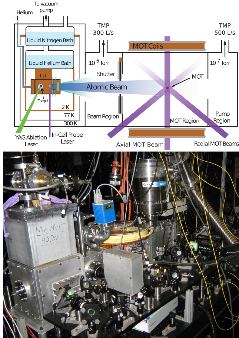
Figure 2.2.2: Schematic and photograph of the apparatus used for the buffer-gas loaded MOTs of atoms. A cryogenic buffer gas beam source (left, labeled 'Mr. MOT 9000') opens into a room-temperature MOT section, separated by a differential pumping region. The photomultiplier tube, which is located transversely to the atomic beam, is visible in the photo as the metal box with lens tube system (photo center, lower). The imaging system, which is also located transversely to the atomic beam, is not visible. The distance between the exit of the cell and the MOT is 42 cm. The MOT coils are visible as the mylar tape-covered wire assembly above the chamber. The lower coil is not visible in the photograph.
