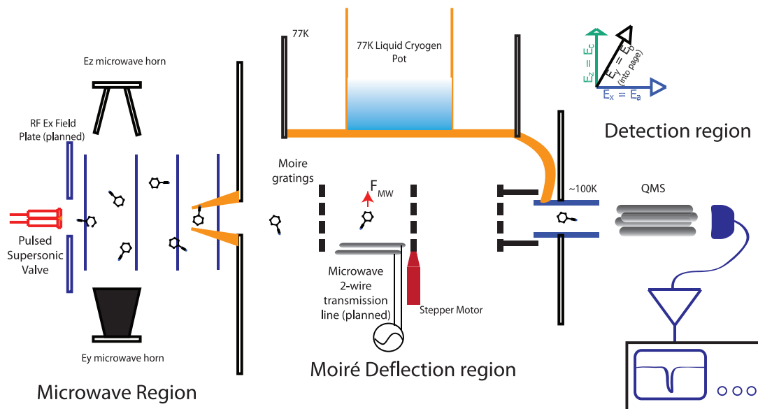
Figure 6.1.7: A schematic of the Moiré deflectometer. Depicted here is the coherent population transfer set-up in the microwave region. After preparation of the desired rotational state, molecules pass through the deflection gratings in the 'closed state,' where only the state of interest is deflected through the gratings by the near resonant microwave or DC electric field generated from the transmission line. Successfully deflected molecules enter the detection region where they are ionized, mass filtered, and detected with an electron multiplier.
