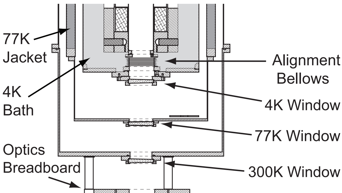
Figure 3-2: Heat sinking of optical access windows. The alignment bellows completes the IVC vacuum space by joining the lower IVC to the 4K cold plate.
