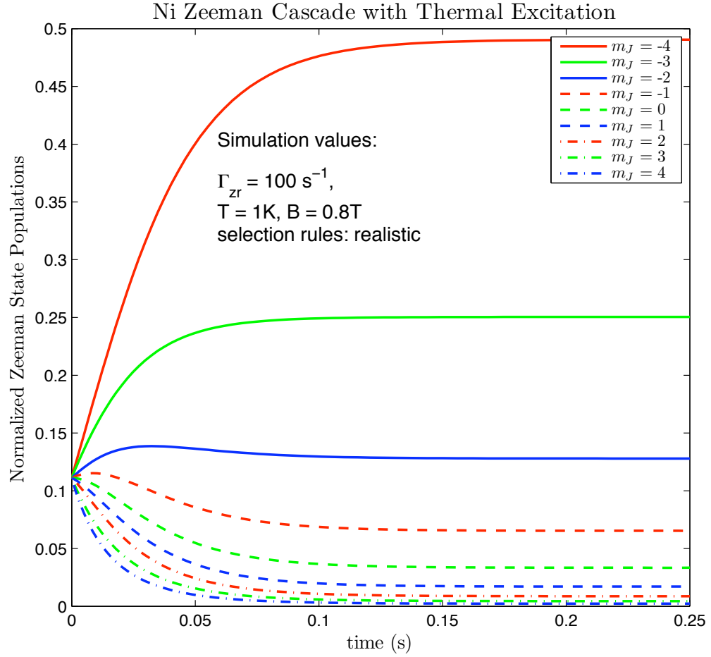
Figure 2-7: Nickel Zeeman cascade with thermal excitation assuming realistic selection rules listed in Table 2.1. The atoms are at T = 1\text{K}, B = 0.8\text{T} . The MLFS state relaxation rate is \Gamma_{zr} = 100 \text{ s}^{-1} . The t = 0 decay rate of the MFLS state is now \sim 2/3 \Gamma_{zr} . The approach to thermal equilibrium is faster than the case when \Delta m_J = \pm 1 , but slower than the case when all transition rates are equal.
