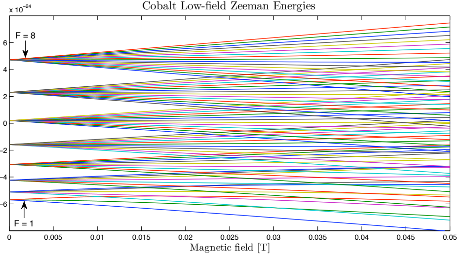
Figure 4-1: Zeeman structure of Cobalt at low-field. F is a good quantum number at very low fields. As the interaction with the external field becomes on the same order as the hyperfine interaction levels start to cross and F is no longer a good quantum number.
