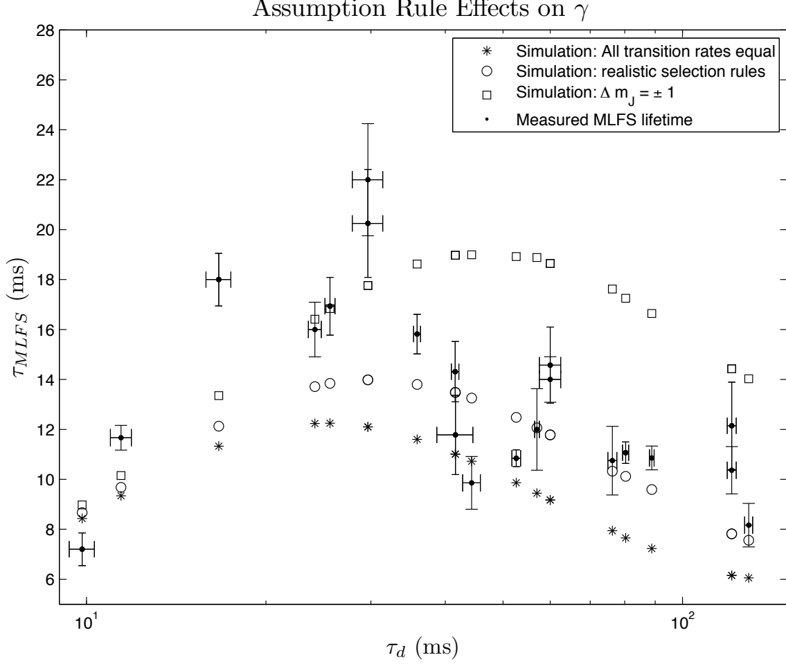
Figure 4-14: Effects of assumed selection rules on \gamma . The effect of collisional excitation on the value of \gamma depends upon which selection rules are assumed. Although we have guidance from the literature [27, 44] on realistic selection rules, we do not know them for sure. We use the extremes in selection rules ( \Delta m_J = \pm 1 ; all transition rates are equal) to set a lower bound of \gamma > 2 \times 10^3 .
