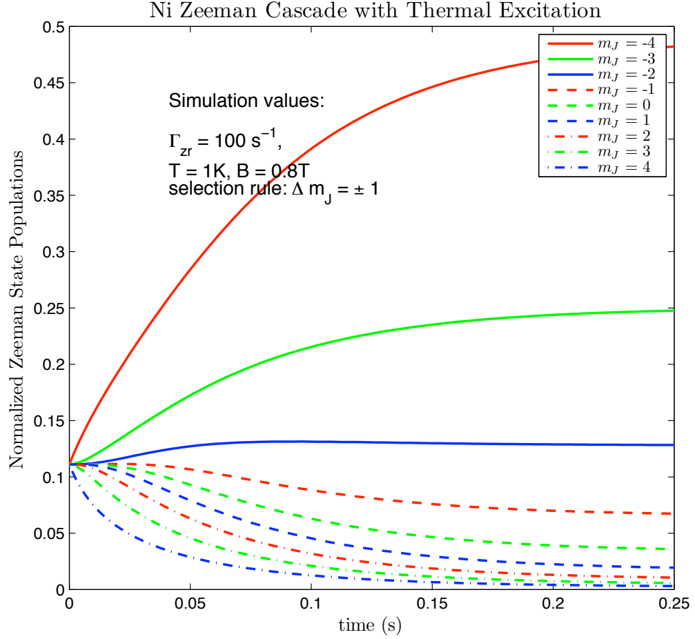
Figure 2-6: Nickel Zeeman Cascade with thermal excitation at T = 1\text{K} , B = 0.8\text{T} assuming \Delta m_J = \pm 1 and a Zeeman relaxation rate of 100 \text{ s}^{-1} . The t = 0 decay rate of the MFLS has decreased by a factor of two from the true Zeeman relaxation rate. The approach to thermal equilibrium is slower than the case where all Zeeman transition rates are assumed to be equal because the initial decay and growth rates are lower.
