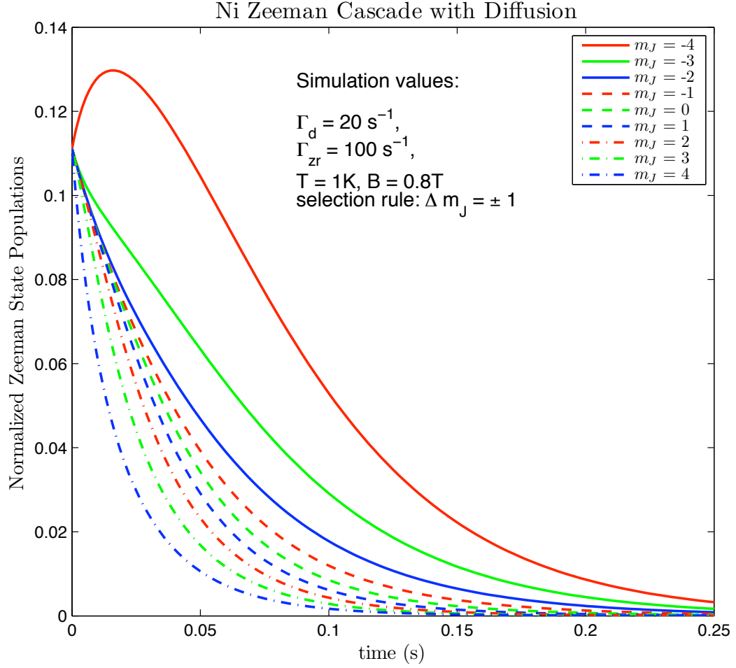
Figure 2-9: Nickel Zeeman cascade with thermal excitation and diffusion at T = 1\text{K} , B = 0.8\text{T} . The MLFS state relaxation rate is \Gamma_{zr} = 100 \text{ s}^{-1} and the diffusion rate is 20 \text{ s}^{-1} . A thermal distribution is established as the atoms diffuse to the cell walls. Initially the MHFS state population grows. After several Zeeman relaxation lifetimes MHFS atoms diffuse to the wall at the diffusion rate.
