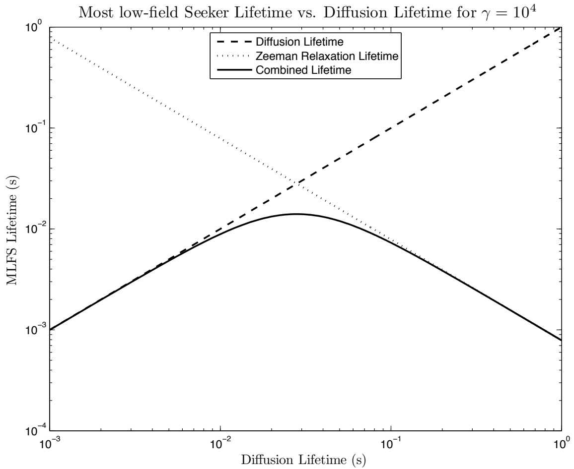
Figure 2-1: Simple MLFS Lifetime vs. Diffusion Lifetime Model. Dotted lines denote pure Zeeman relaxation and diffusion losses. This model assumes no thermal excitation occurs.
