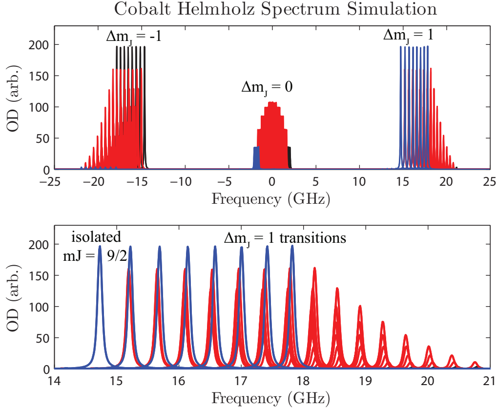
Figure 4-3: Cobalt in 1T Helmholz Field. Transitions from the m_J = J ( m_J = -J ) states are in blue(black). The m_J = J line is split into several lines corresponding to different values of m_I . There is only one m_J = J state transition that does not overlap with any other spectral line. Due to the large multiplicity of transitions in cobalt, the OD of the isolated transition will be lower at a given density than the m_J = J lines in Fe and Ni.
