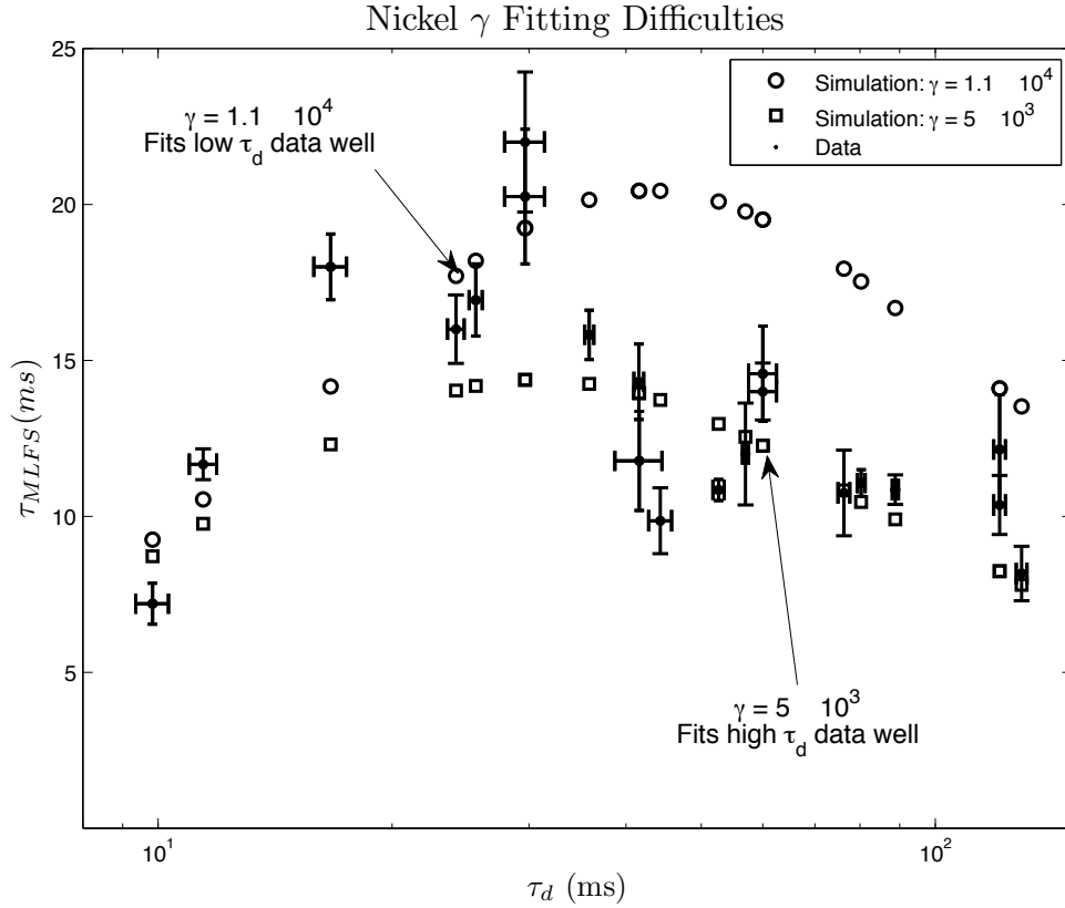
Figure 4-12: It is not possible to find a value of \gamma that fits both the low \tau_d and high \tau_d regions of our data. There may be a systematic effect not fully understood that causes a deviation from the model in one of the regimes. This effect creates an uncertainty of a factor of 2 in the final value of \gamma .
