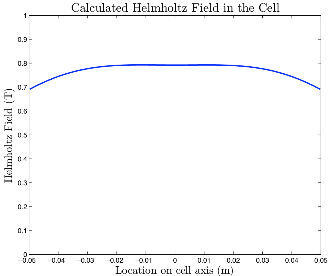
Figure 3-3: Plot of the variation of field within the cell in the Helmholtz magnet configuration. The variation of field with position introduces magnetic broadening on the observed spectra.
