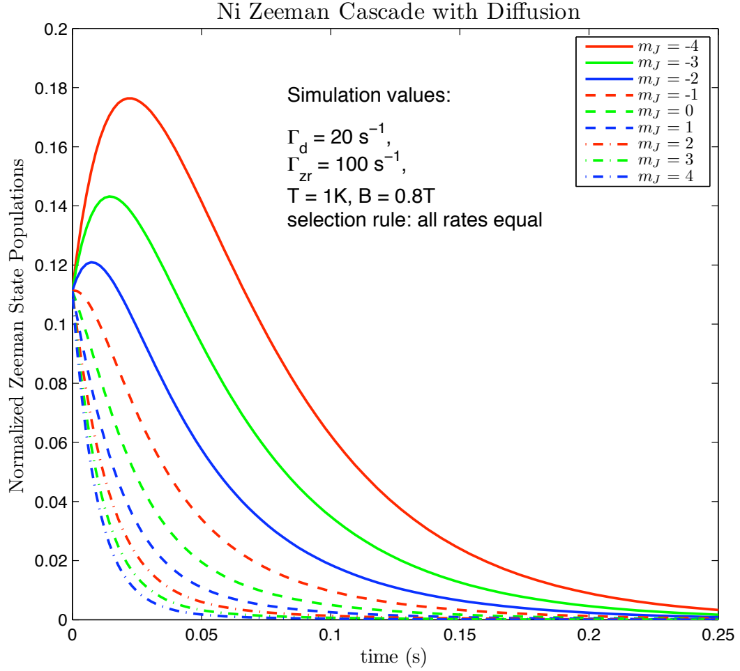
Figure 2-8: Nickel Zeeman Cascade at T = 1\text{K} , B = 0.8\text{T} assuming Zeeman relaxation rates are equal for all transitions. The MLFS decay at \Gamma_{zr} = 100 \text{ s}^{-1} and the diffusion rate is 20 \text{ s}^{-1} . A thermal distribution is established as the atoms diffuse to the cell walls.
