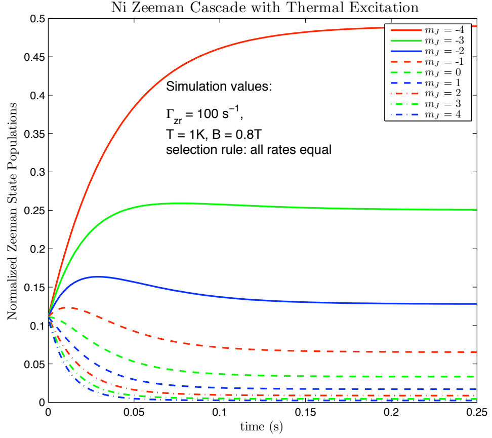
Figure 2-5: Nickel Zeeman Cascade with thermal excitation at T = 1\text{K} , B = 0.8\text{T} assuming equal Zeeman relaxation rates for all transitions and a rate of 100 \text{ s}^{-1} for the MLFS state. When thermal repopulation occurs in addition to Zeeman relaxation, the Zeeman populations obey a Boltzmann distribution as t \rightarrow \infty .
