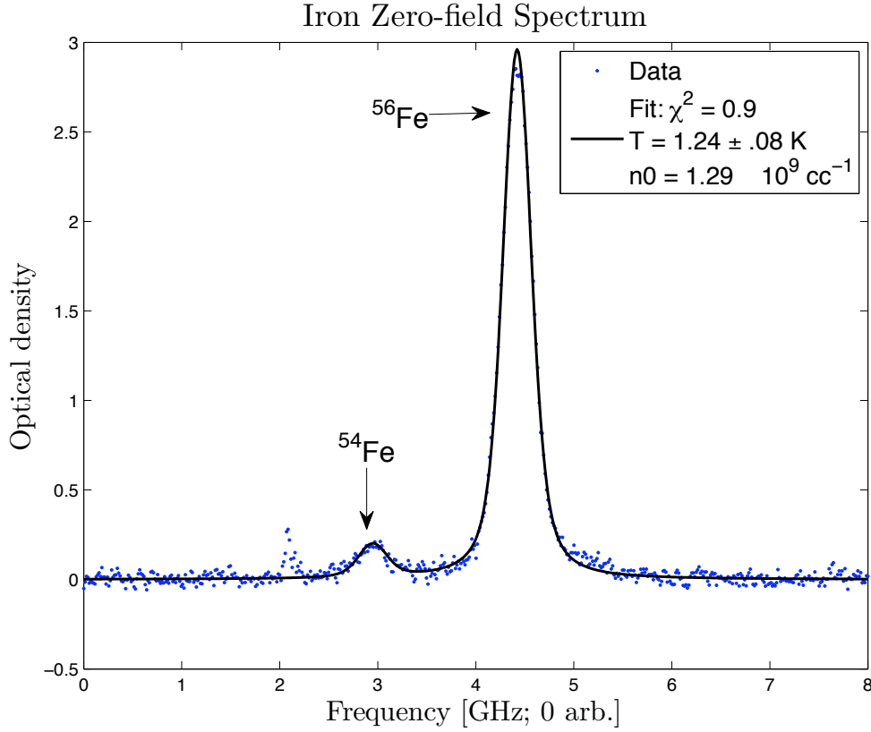
Figure 4-15: Zero-field Iron spectrum fit for density and temperature. Temperature is obtained by fitting a Voigt profile to the spectrum.
