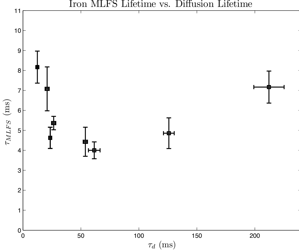
Figure 4-17: Iron MLFS lifetime versus Diffusion Lifetime. There is no region of \tau_d for which \tau_{MLFS} increases. This indicates that Zeeman relaxation loss dominates diffusion loss for all observed values of \tau_d and we can set an upper limit of \gamma < 5 \times 10^3 .
