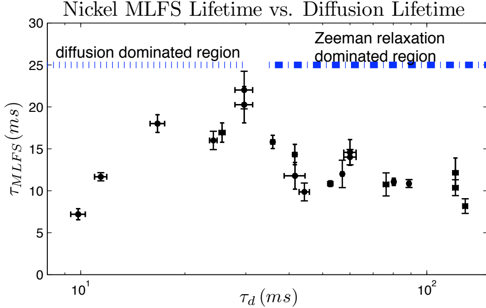
Figure 4-7: Nickel \tau_{MLFS} vs. \tau_d . We observe a region at low \tau_d where the MLFS state lifetime increases with \tau_d , a signature of diffusion to the walls. As \tau_d increases to \sim 30 ms the Zeeman relaxation rate equals the diffusion loss rate. Increasing \tau_d beyond this point causes the measured \tau_{MLFS} to decrease.
