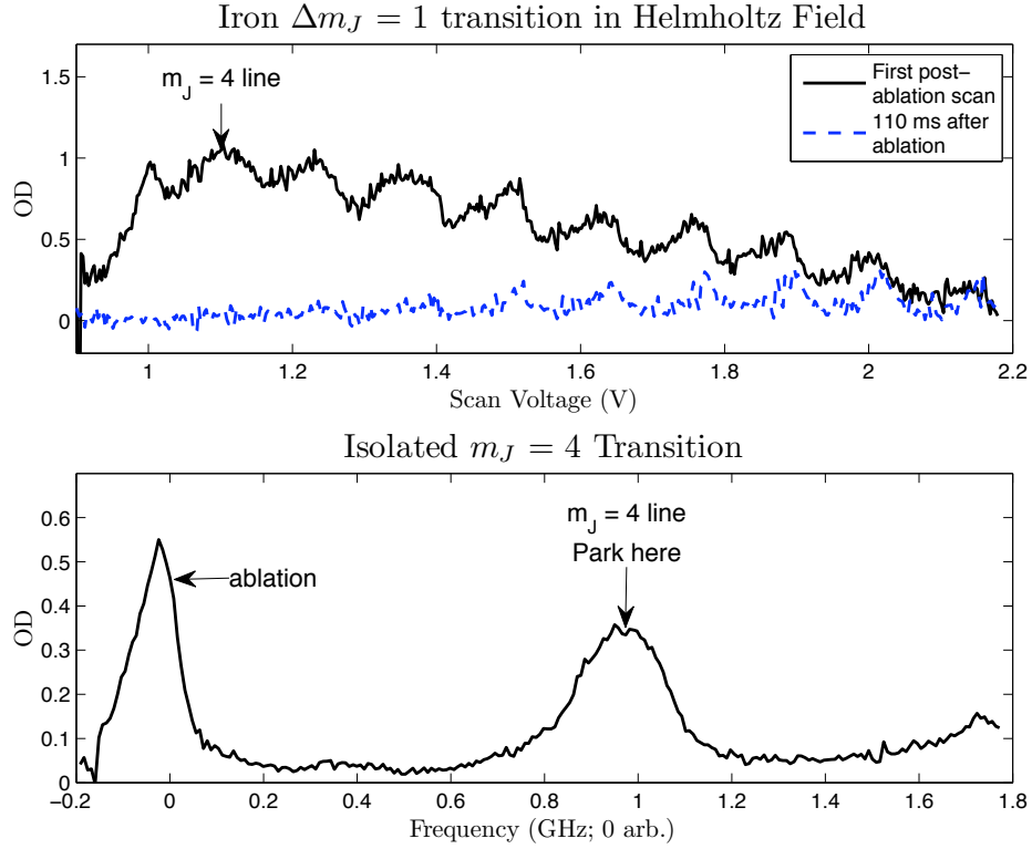
Figure 4-16: Iron Observed Spectrum in 0.5 T Helmholtz Field. The top figure shows a spectrum immediately after ablation and another \sim 100 ms after ablation. The m_J = 4 population has decayed away completely. In the bottom plot the laser scan range has been decreased to isolate the m_J = 4 peak. The laser is tuned to the peak of the resonance to measure the decay of the MLFS state population decay.
