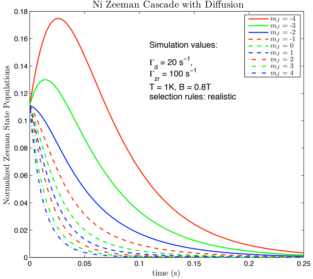
Figure 2-10: Nickel Zeeman cascade with thermal excitation and diffusion assuming realistic selection rules listed in Table 2.1. The atoms are at T = 1K, B = 0.8T . The MLFS state relaxation rate is \Gamma_{zr} = 100 s^{-1} and the diffusion rate is 20 s^{-1} . The behavior falls somewhere between the two extreme cases previously discussed. Only the two most high field seeking states experience growth; all other states begin to decay immediately.
