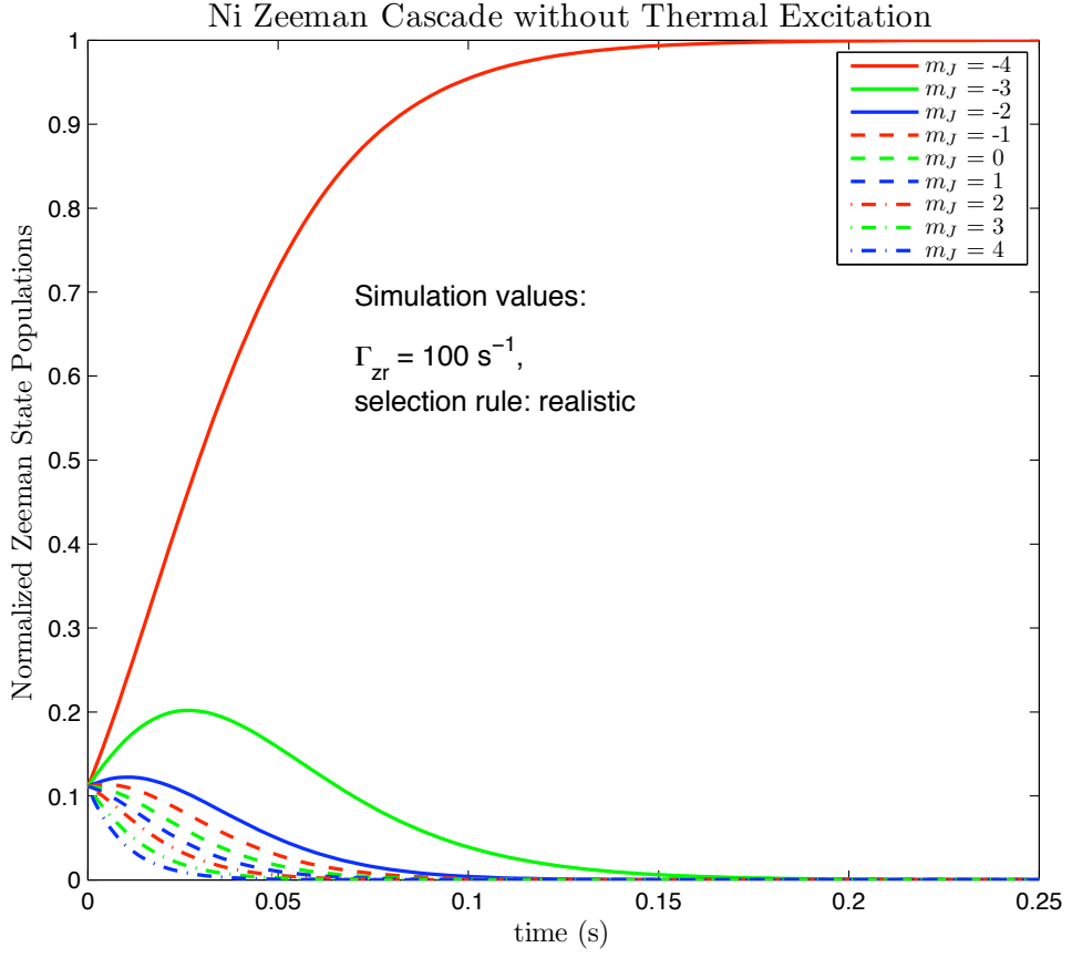
Figure 2-4: Nickel Zeeman cascade without thermal excitation assuming realistic selection rules listed in Table 2.1. The MLFS state relaxation rate is \Gamma_{zr} = 100 \text{ s}^{-1} . The approach to steady state is faster than the case when all transition rates are equal, but slower than the case when \Delta m_J = \pm 1 .
