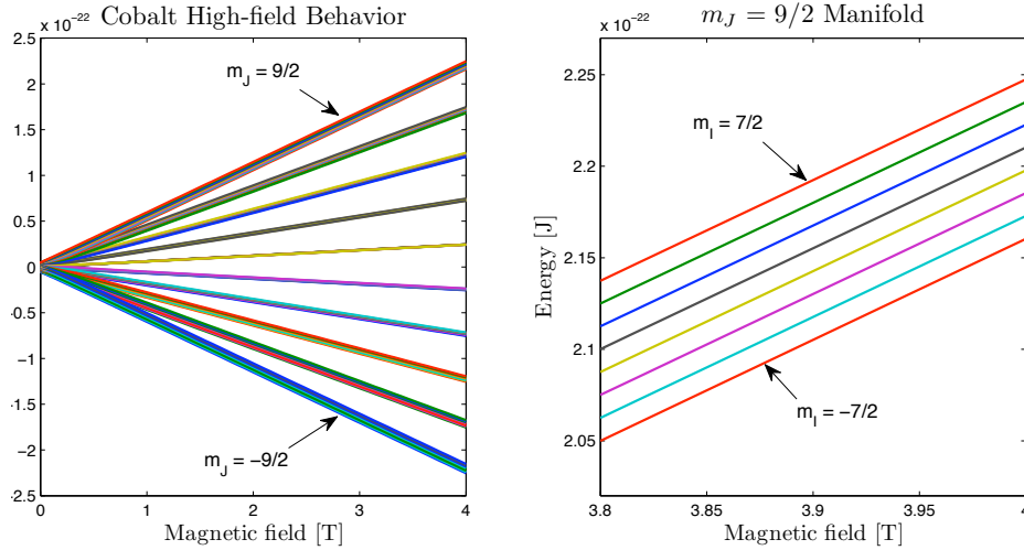
Figure 4-2: Zeeman structure of Cobalt in high magnetic fields. The energy splittings are dominated by projection of the electronic angular momentum onto the external field so J is a good quantum number. Each of the 10 m_J manifolds contain 8 states corresponding to different values of m_I . The linewidths of the above spectra include only the natural linewidths. In our experiment we have additional Doppler and magnetic broadening. The observed linewidths are \sim 200 - 300 MHz.
