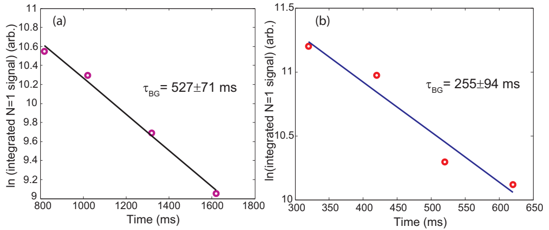
Figure 3.15: Signals of CaF ( N = 1 ) integrated over 210 ms as a function of time after ablation at which the detection laser is switched on. (a) Data taken when the flow is 0.5 sccm and shutter is actuated at 0.5 Hz (YAG repetition rate) with an opening duration of 100 ms. (a) Data taken when the flow is 0.75 sccm and shutter is actuated at 1 Hz (YAG repetition rate) with an opening duration of 100 ms.
