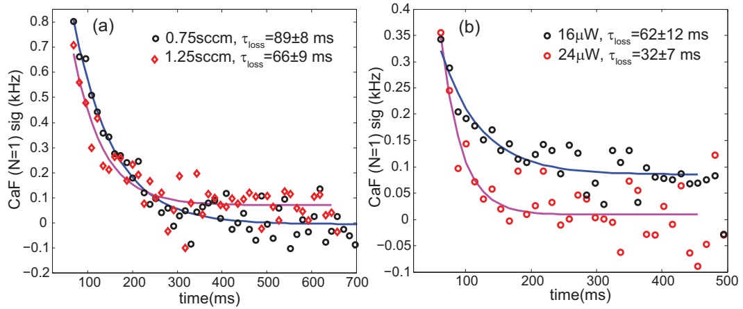
Figure 3.12: (a) Time decay of trapped CaF ( N = 1 ) signals for two buffer-gas flows. Detection power is fixed at 15 \mu\text{W} ; Yag at 1 Hz. (b) Time decay of CaF( N = 1 ) signals for two detection powers. Flow is fixed at 1.25 sccm; YAG at 1 Hz.
