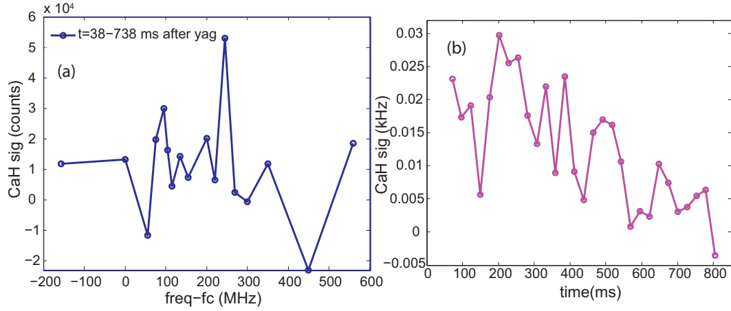
Figure 3.19: (a) Spectrum of loaded CaH ( N = 0 ) using (B_1, B_2) = (3.5, 1.5) T. Experiment parameters: 0.75 sccm without shutter; YAG (5mJ) at 1 Hz; 1st OPL (polarization parallel to the magnetic field) on between 0 – 17 ms. 2nd OPL is \sigma_+ polarized. (b) Average time decay signal of CaH over the spectrum.
