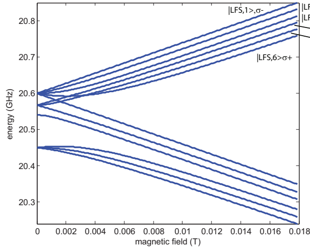
Figure 6.3: Calculated Zeeman level of CaF X^2\Sigma^+(N=1) based on Eq. 6.5. The basis states are |N, S, J, F, m_F\rangle . Here, we assign the six LFS states to |\text{LFS},1\rangle - |\text{LFS},6\rangle in order of decreasing energies.
