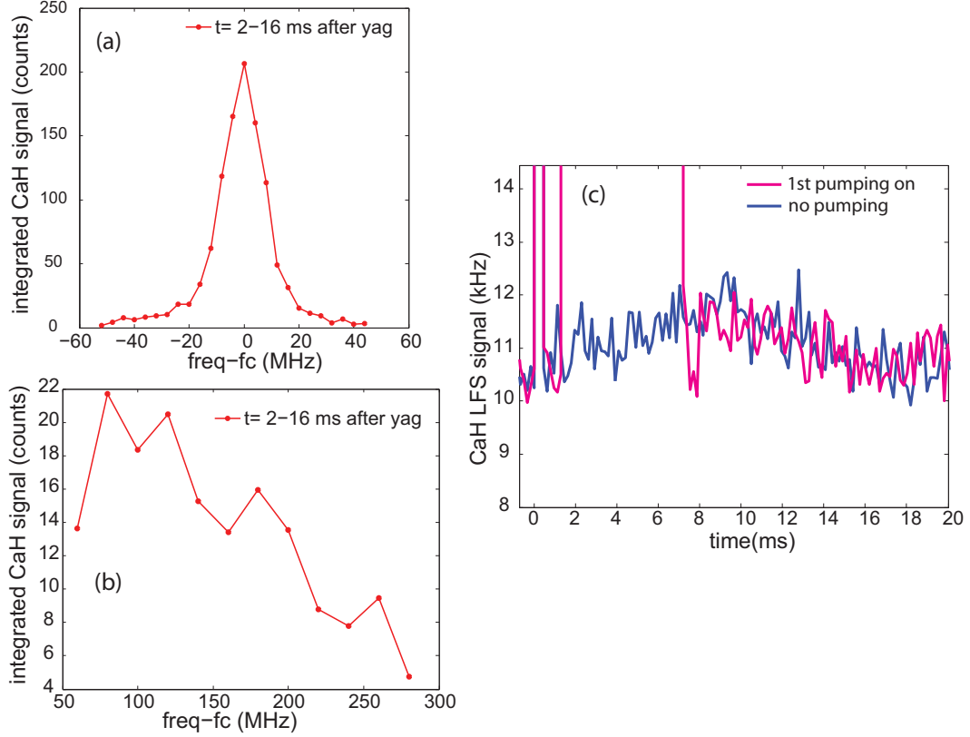
Figure 3.18: (a) and (b) plot the CaH (LFS) beam spectrum at zero field and 3.5 T. (c) LFS signals with and without the 1st OPL turning on. Trap is at 3.5 T.
