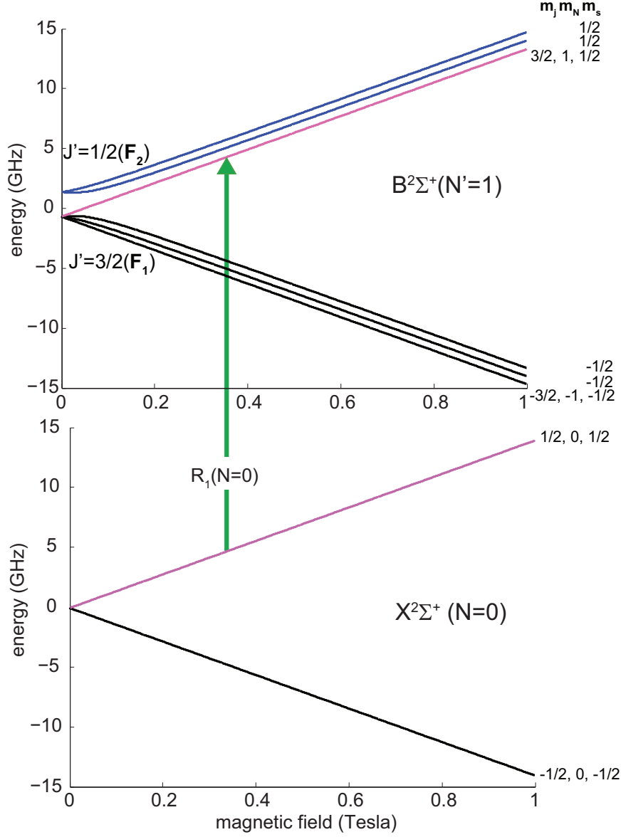
Figure 3.17: Calculated CaF Zeeman levels for the R_1(1/2) line of the X-B transition. Here, we only consider H = \gamma_v \vec{N} \cdot \vec{S} - \vec{\mu}_S \cdot \vec{B} . For B^2\Sigma^+ , \gamma_{v'=0} = -0.04581 \text{ cm}^{-1} = -1.37 \text{ GHz} [61].
