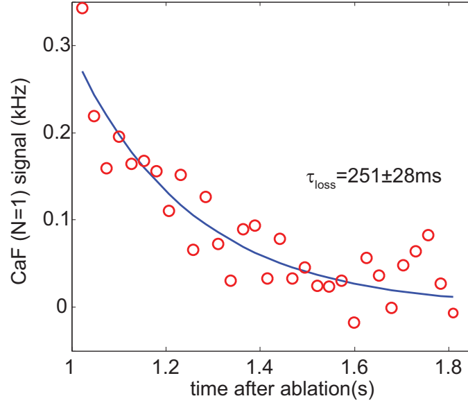
Figure 3.14: Trapped CaF ( N = 1 ) signal after the shutter is closed. The detection laser is turned on at 1 s. Flow = 0.5 sccm; Shutter actuated at 0.5 Hz (same with YAG repetition rate) with an opening duration of 100 ms.
