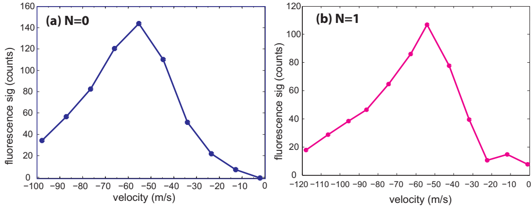
Figure 2.23: Longitudinal velocity distribution of CaF in N = 0 (a) and N = 1 state (b). N = 1 is detected via the R_1(3/2) = 564.642474 \text{ THz} line of the X - B transition. YAG energy is 5 mJ at 2Hz; flow is 1.25 sccm.
